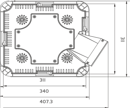
Size Diagram of Forme 4 Model
