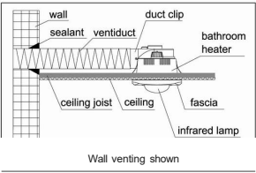
Wall venting shown
